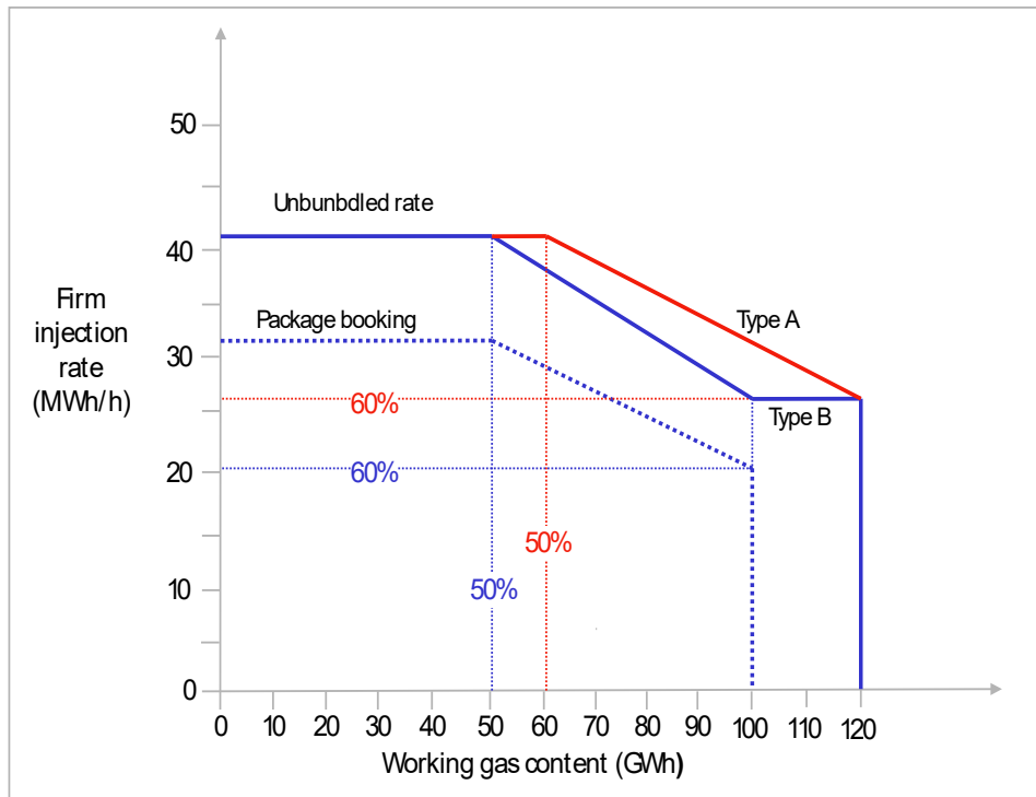
Example: Firm injection rate curve (bundled + unbundled)
